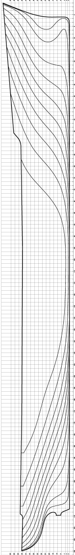
SHEER PLAN
